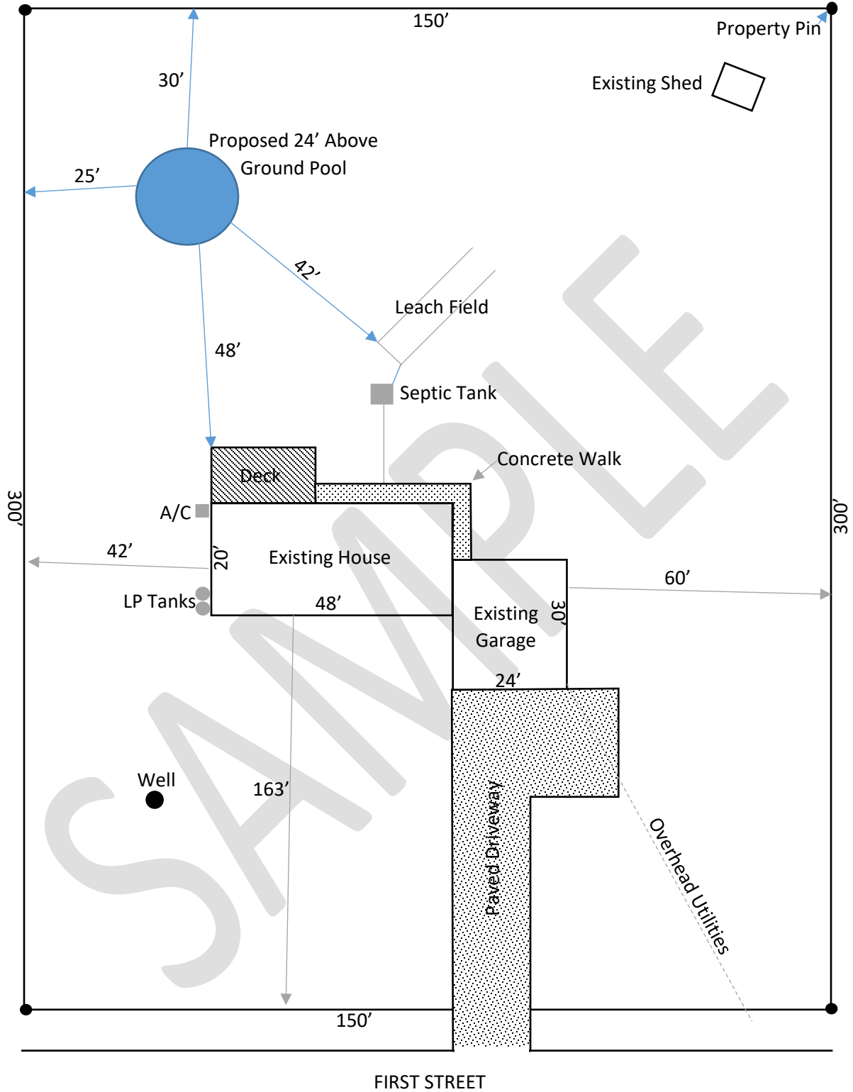
Site Plan – John Smith, 123 First Street. Proposed 24' Round Above Ground Pool
