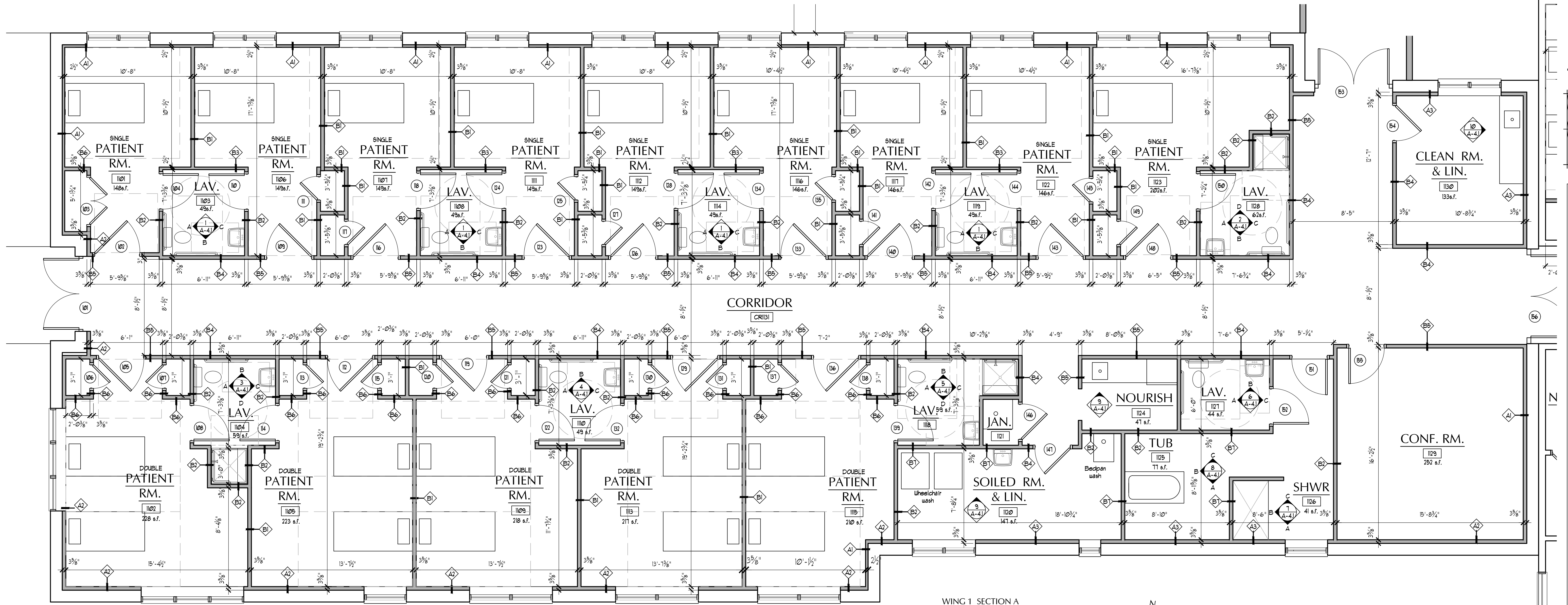
1 WING 1 SECTION A FIRST FLOOR PLAN SCALE: 1/4"=1'-0"
