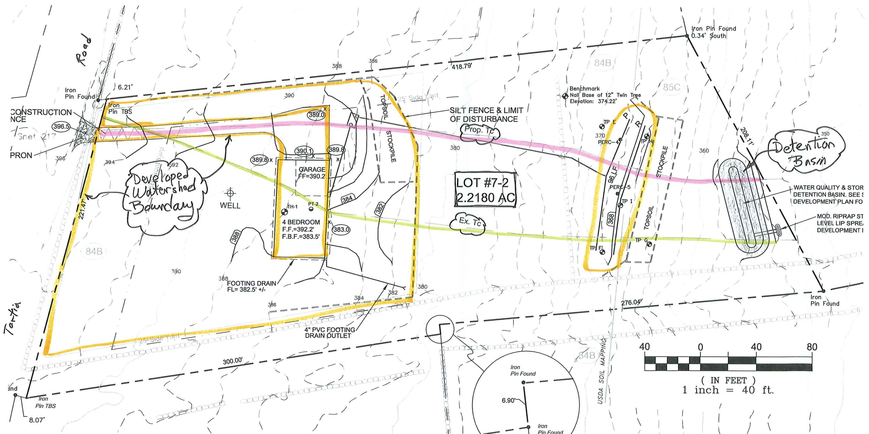
Watershed Map - Lot 7-2
