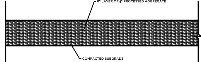
LANDING AREA DETAIL
