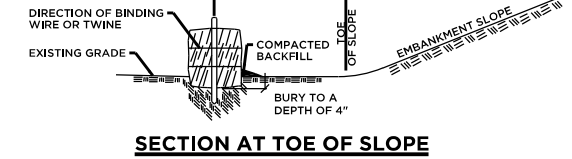
SECTION AT TOE OF SLOPE
