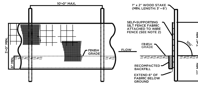
ELEVATION SECTION
