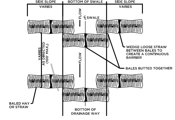
PLAN SECTION AT SWALE
