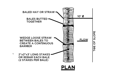
PLAN SECTION AT TOE OF SLOPE
